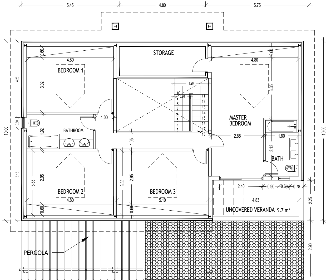
HOUSE 170 SOUNI ATTIC PLAN SC 1:100
