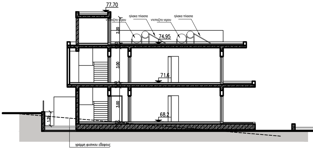
section B-B
